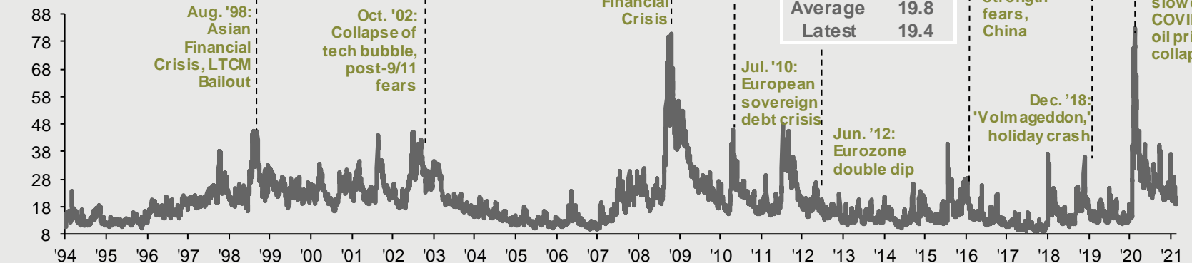
VIX Index
